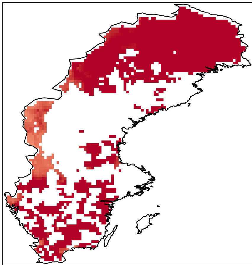
DI6 and river discharge
